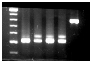
Psf3
