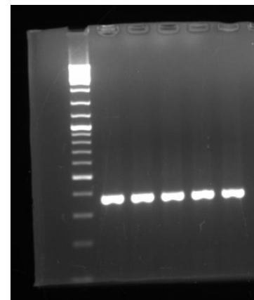
Actin
