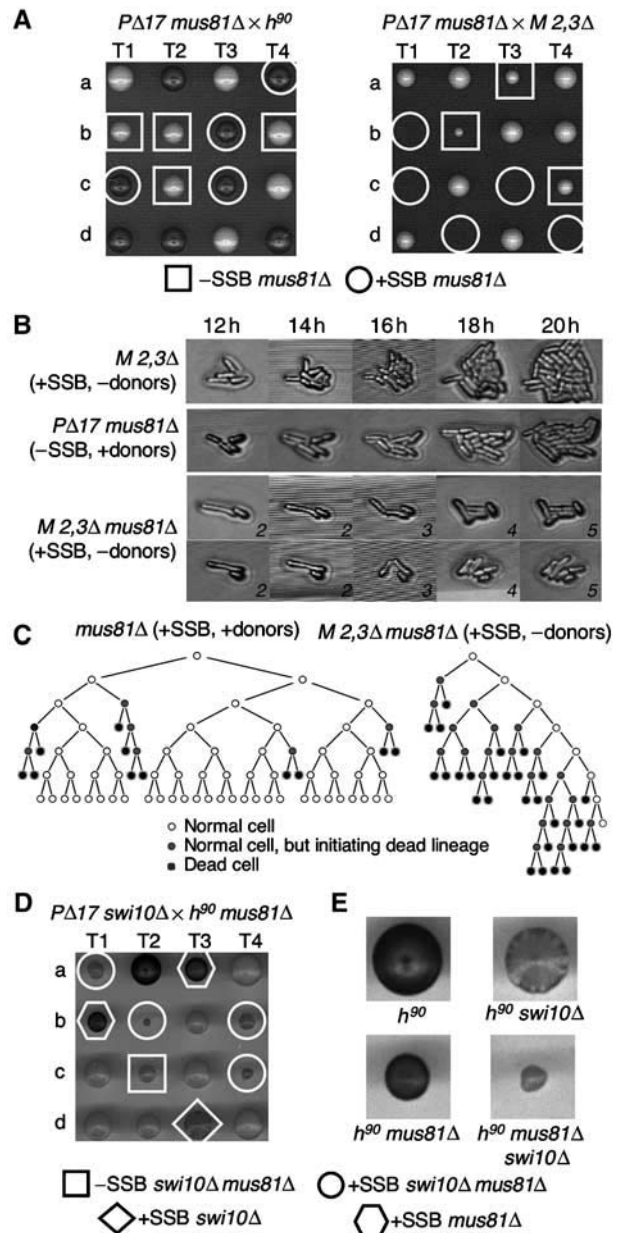
Figure 3 Mus81 is essential for sister chromatid recombination. (A) Tetrads dissections of PΔ17 mus81Δ crossed with h 90 (left) or M(2,3Δ) (right). The circles and the squares surround mus81Δ mutants with ( h 90 or M(2,3Δ) ) or without ( PΔ17 ) SSB, respectively. (B) Time course of germinating wild type and mus81Δ mutants with ( M(2,3Δ) ) or without ( PΔ17 ) the SSB. Numbers of cells are indicated for mus81Δ M(2,3Δ) mutants. (C) Pedigree of the mus81Δ mutant with or without donors. The empty circles indicate dividing cells, the grey circles indicate elongated cells and the black circles indicate undividing cells. (D) Tetrads dissections of h 90 mus81Δ crossed with PΔ17 swi10Δ . A circle, rhombus or hexagon surrounds mutants of interest with the SSB ( h 90 or M(2,3Δ) ), whereas squares surround mutants without the SSB ( PΔ17 ). (E) Iodine staining of wild-type, swi10Δ , mus81Δ and swi10Δ mus81Δ h 90 colonies, after 4 days at 33°C and 4 days at 25°C.
