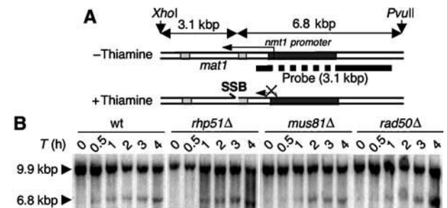
Figure 5 Break formation in mat1P:nmt1:KAN (2,3Δ) strains. (A) Schematic representation of the MT locus in the mat1P:nmt1:KAN (2,3Δ) strain. The strong nmt1 thiamine repressible promoter (dark grey box) was inserted just distal to mat1 (Holmes et al , 2005). The transcript is turned on (-thiamine) and the break is repaired at mat1 . When the promoter is turned off (+thiamine), one can follow the timing of break formation. The size (in kbp) of the XhoI-PvuII DNA fragments is indicated and the probe is shown. (B) Genomic DNA of wild-type (PB157), rhp51Δ (LR95), mus81Δ (LR27) and rad50Δ (LR164) mutants was digested with XhoI and PvuII and analysed by Southern blot.
