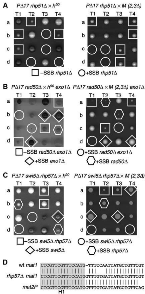
Figure 2 The Rad22A epistasis group is essential for MT switching and sister chromatid recombination. (A) Tetrads dissections of PΔ17 rhp51Δ crossed with h 90 (left) or with M(2,3Δ) (right). (B) Tetrads dissections of PΔ17 rad50Δ crossed with h 90 and M(2,3Δ) exo1Δ mutants. (C) Tetrads dissections of PΔ17 swi5Δ crossed with h 90 and M(2,3Δ) rhp57Δ mutants. A circle, rhombus or hexagon surrounds mutants of interest with the SSB ( h 90 or M(2,3Δ) ), whereas squares surround mutants without the SSB ( PΔ17 ). (D) Alignment of mat1 distal and mat2P distal sequences from wild type and rhp57Δ variants with a stable MT locus.
