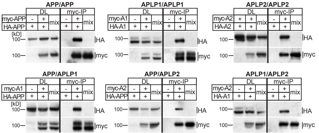
Supplementary Fig. 1: Homo- and heterotypic interactions of APP and APLPs APP family protein interaction was analyzed by coimmunoprecipitation experiment as described in Fig. 1. Here, the reverse experiments were performed. For this purpose, the myc-tagged APP/APLP constructs were immunoprecipitated with anti-myc-Agarose and immunoblotted for the co-expressed corresponding HA-tagged APP/APLPs. Both, homo- and heterotypic interactions of APP family proteins were independent from the tag used.
